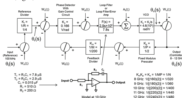
8. Specific PLL Block Diagram & Phase Noise Propagation Model at 10-GHz mid-band output for 8- to 12-GHz output/50-MHz step PLL frequency synthesizer.
