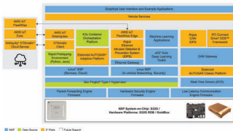
2. GoldVIP utilizes Kubernetes K3s for container orchestration. Two separate AWS services manage edge runtime and cloud services, with OTA updates handled by the OTAmatic client.
