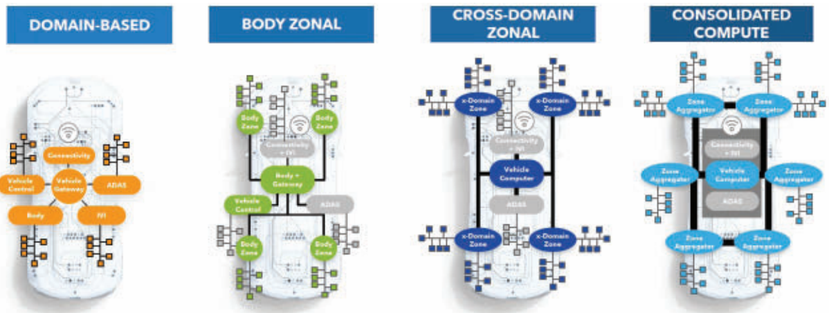
1. Automotive manufacturers are moving toward domain and zonal architectures and away from a disparate array of ECUs.
